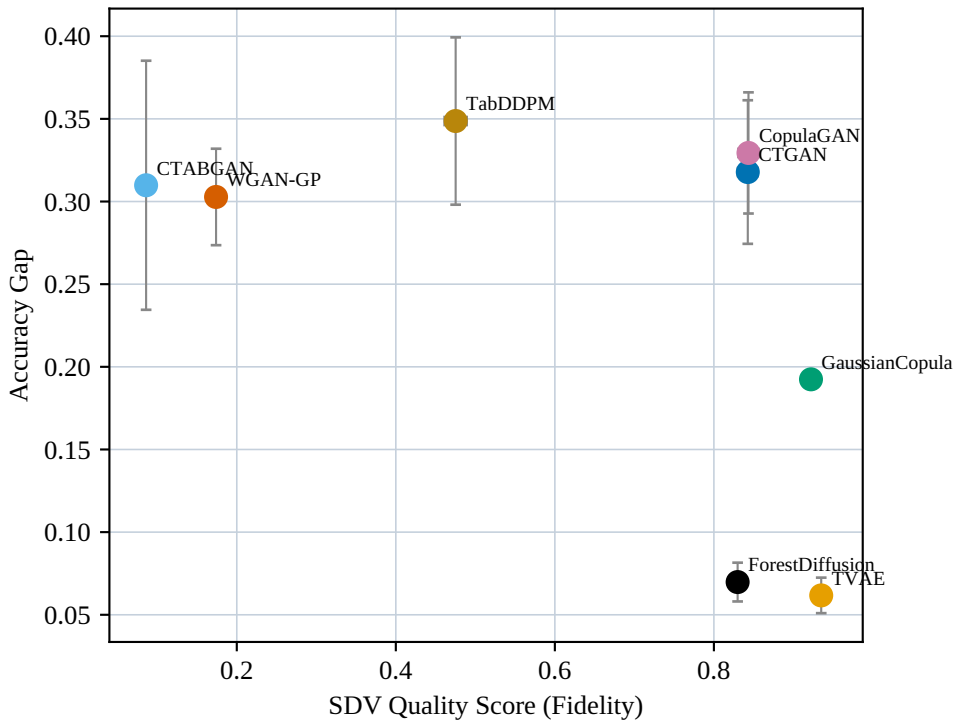
Forest Cover: SDV Quality Score (Fidelity) vs Accuracy Gap
